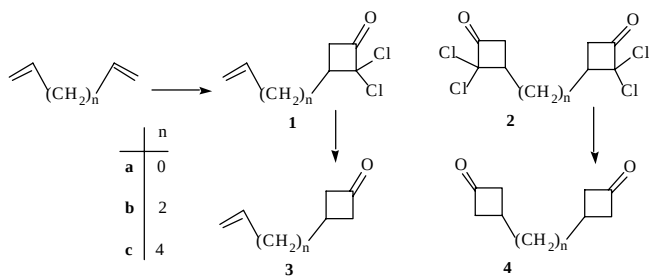
Scheme 1 Preparation of cyclobutanones 3 and 4
