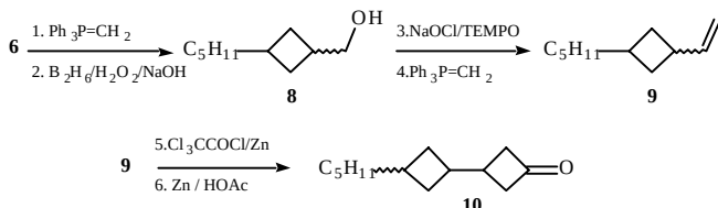
Scheme 4 Synthetic sequence to give compound 10
