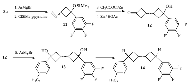
Scheme 5 Preparative sequence for compound 14
